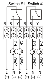
Two SPDT switches Reed switches & terminal strip connection
